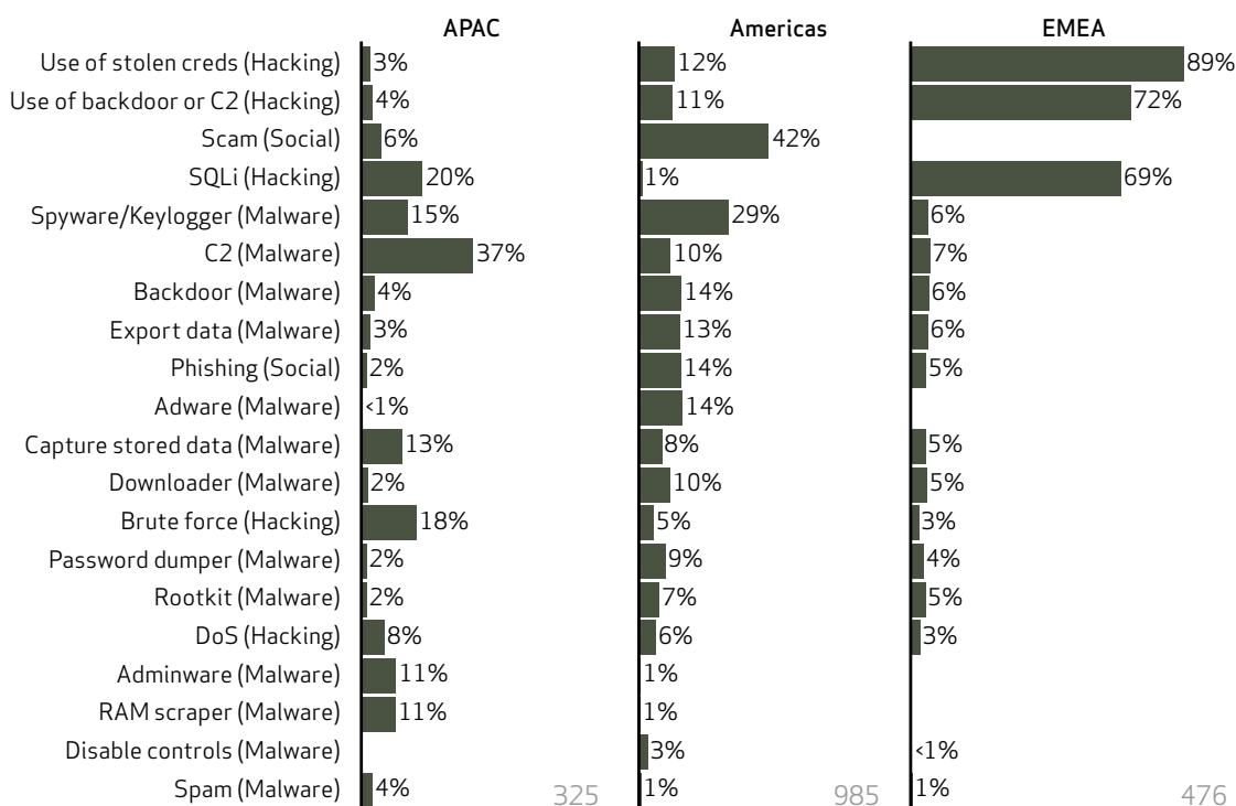
Figure 19: Top 20 threat actions by victim region across 47,000+ security incidents (filtered for network intrusions)
